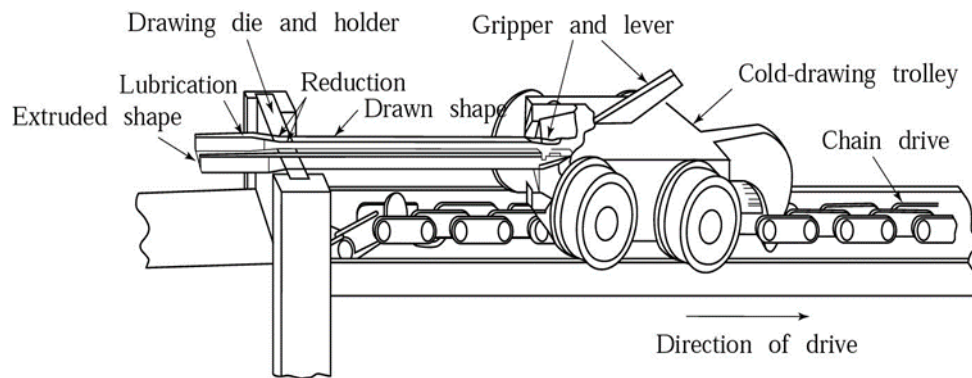
Fig.1: Structural Diagram Of Cold Draw Bench
