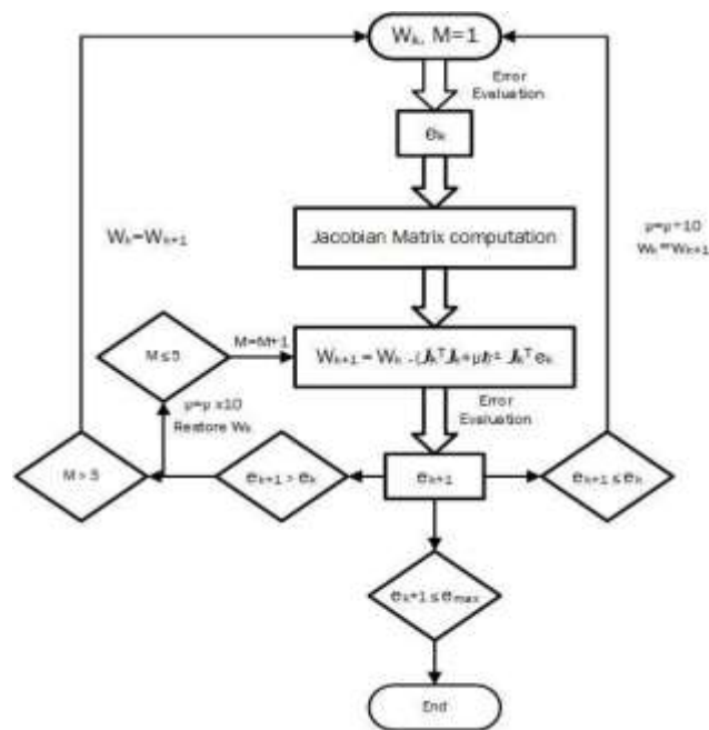
Fig. 1: Block diagram for training using Levenberg–Marquardt algorithm
