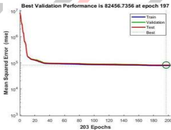
Fig. 10: Neural network performance during training, testing & validation with WT.
