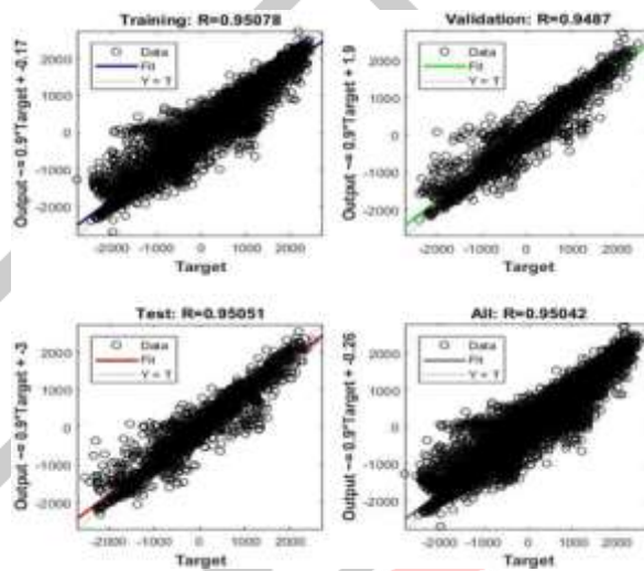
Fig. 9: Regression plot during training, testing & validation for Proposed for Proposed Levenberg-Marquardt (LM) training algorithm with WT.
