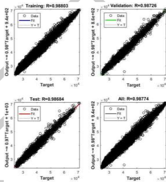
Fig. 12: Regression plot during training, testing & validation for Proposed for Proposed Levenberg-Marquardt (LM) training algorithm without WT.
