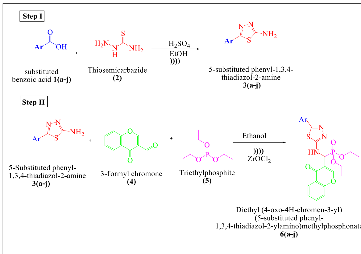
Scheme 1. Scheme Of Synthesis Of Diethyl (4-Oxo-4H-Chromen-3-Yl)(5-Substituted Phenyl-1,3,4-Thiadiazol-2-Ylamino)Methyl Phosphonate Derivatives 6(A-J) .
