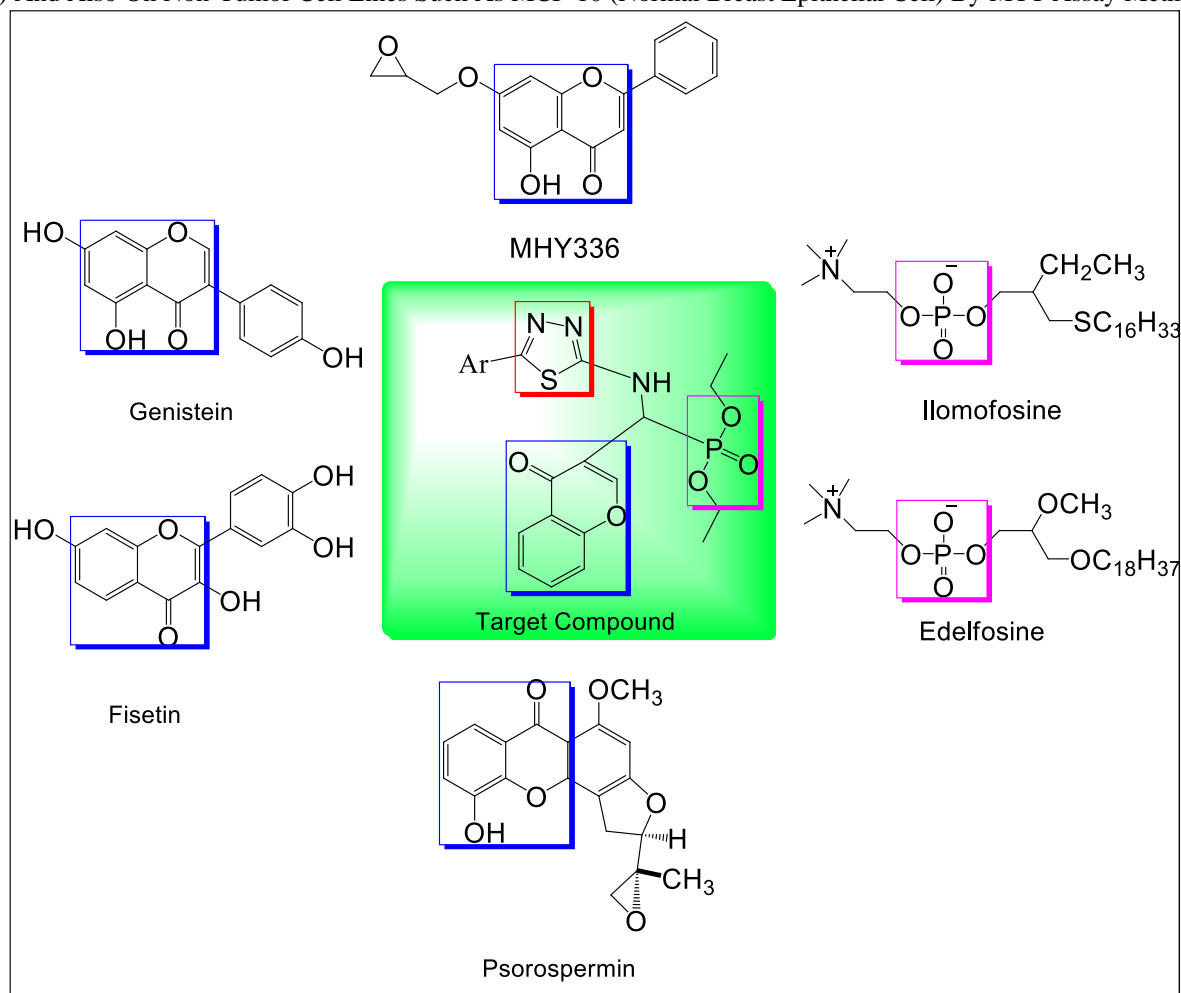
Figure 1. The Designing Protocol For The Target Compound 6(A-J) .
