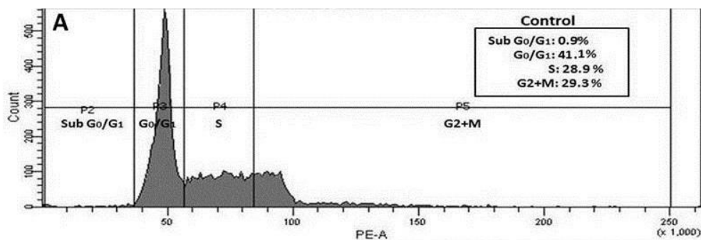
Figure 6. Flow Cytometry Cell Cycle Analysis Of Control And Of Compounds 6h Treated On DU-145 Cancer Cells.
