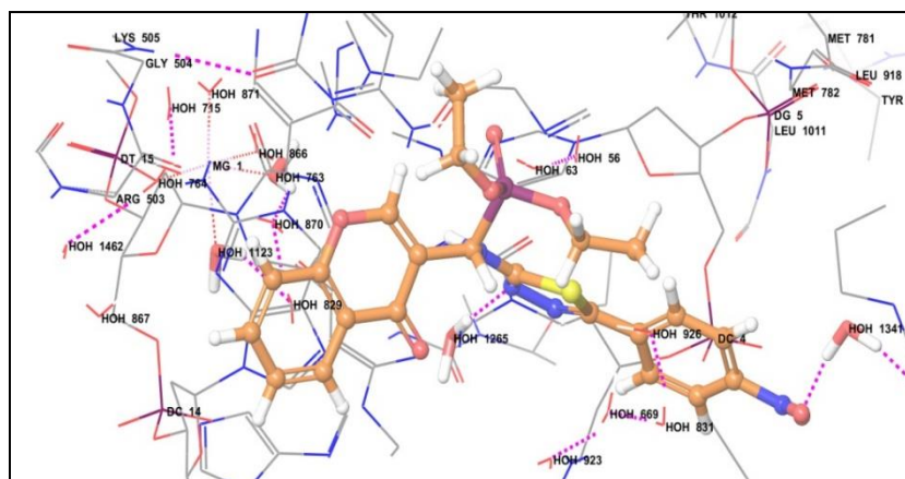
Figure 8. Binding Pose And Molecular Interactions Of 6f Into The Active Site Of Top II A In Silico ADMET Predictions
