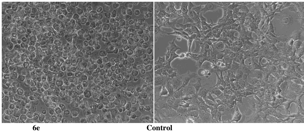
Figure 5. Images For In-Vitro Anticancer Activity Of Compound 6e And Control Against MCF-7 Cancer Cell Line At 100x Magnification
