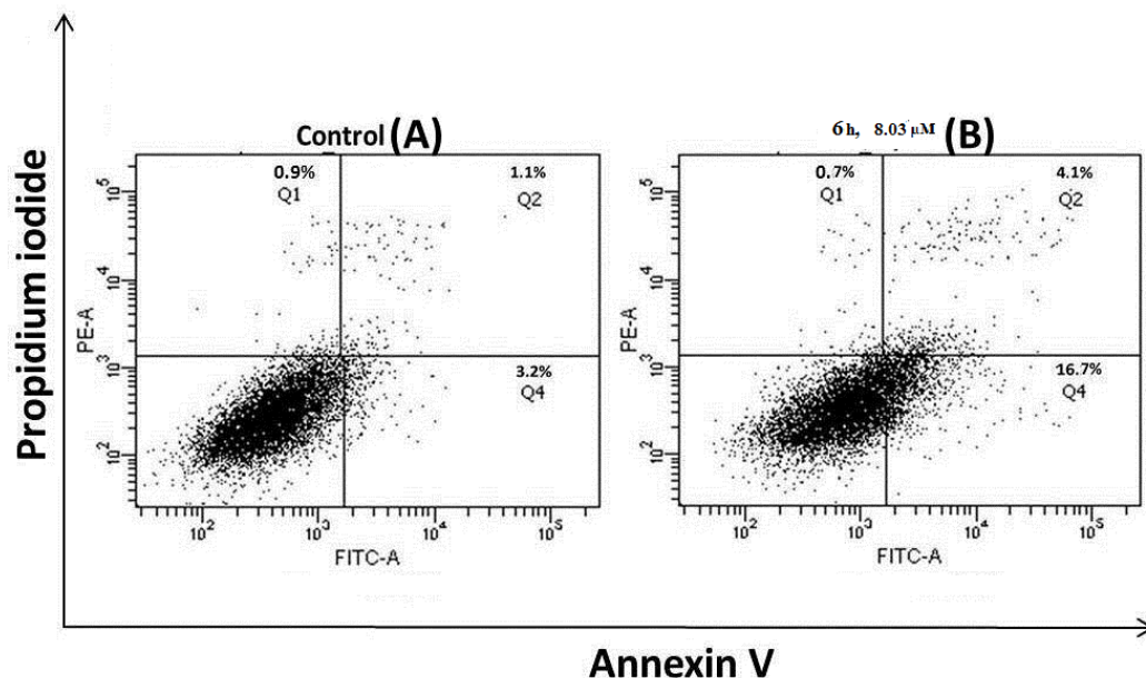
Figure 7. Apoptosis Study By Annexin V/FITC Assay Of Compound 6h .
