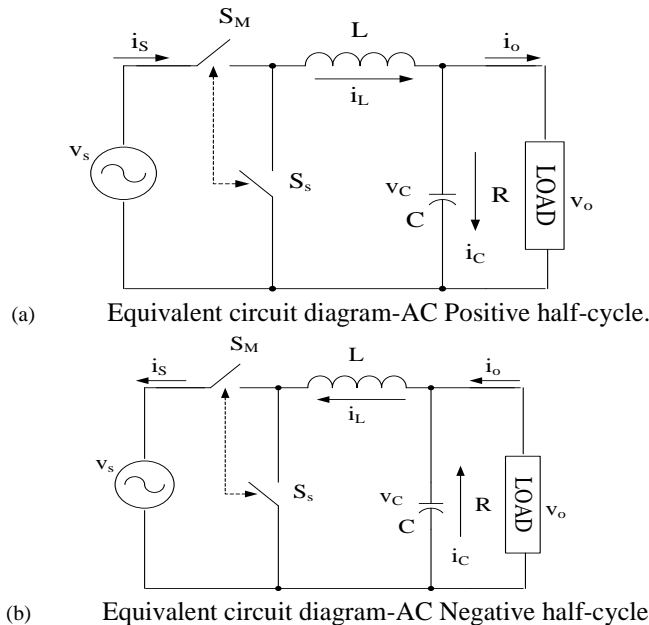
Fig. 3 Buck type DC-modulated AC/AC converter.
