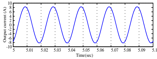
Fig. 11 Output current waveform of AC/AC converter with DC-modulation
