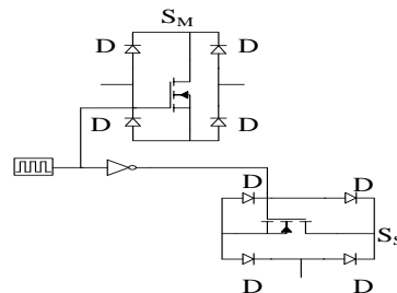
(a) A circuit of bidirectional exclusive switches S_M-S_S .
