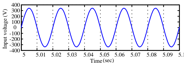
Fig. 9 Input voltage waveform of AC/AC converter with DC-modulation.
