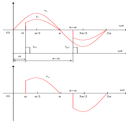
(b) Waveforms
