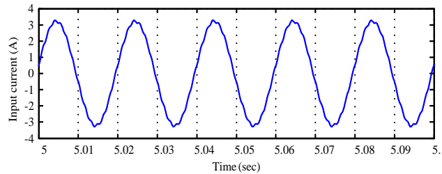
Fig. 12 Input current waveform of AC/AC converter with DC-modulation.
