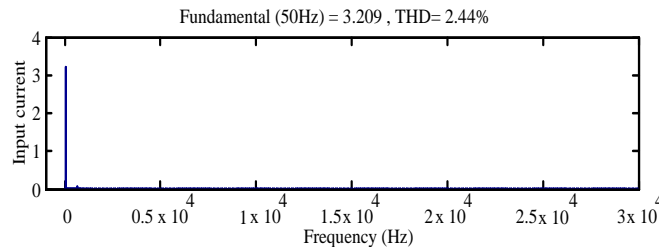
Fig. 15 Harmonic analysis of input current.
