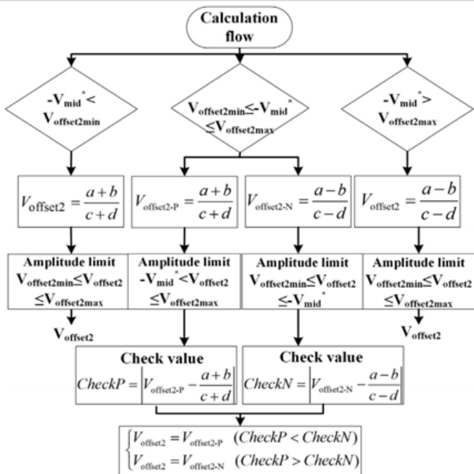
Fig. 14. The calculation flow of V_{offset2}
