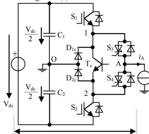
Fig. 3. Multilevel switching cells. (a) 3L–Bidirectional–Vienna (BV) topology.
