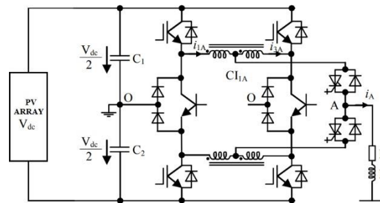
Fig.13 PV inverter with MPPT control
