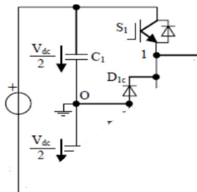
Fig.5 3L-BV Switching Cell
