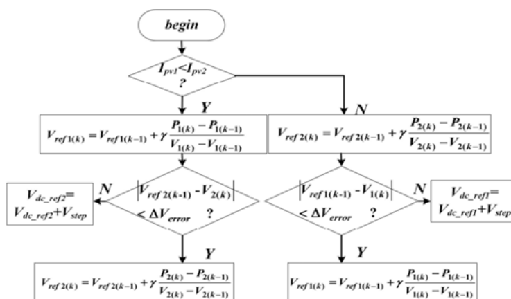
Fig. 15. The algorithm flowchart of independent MPPT control
