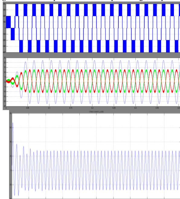
Fig.25 Armature current of induction motor
