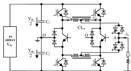
Fig.1, series-connected photovoltaic
