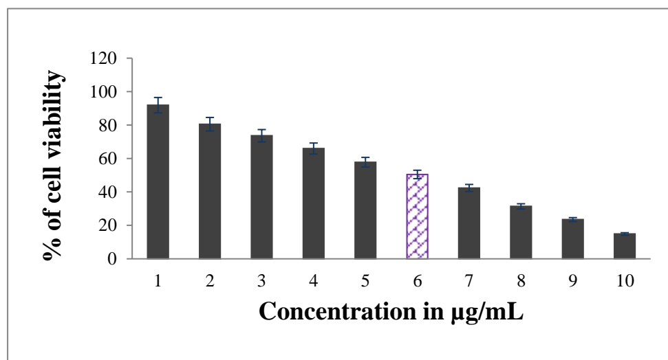
Fig. 5: Cytotoxicity of m-NBTSC against A549 cells
